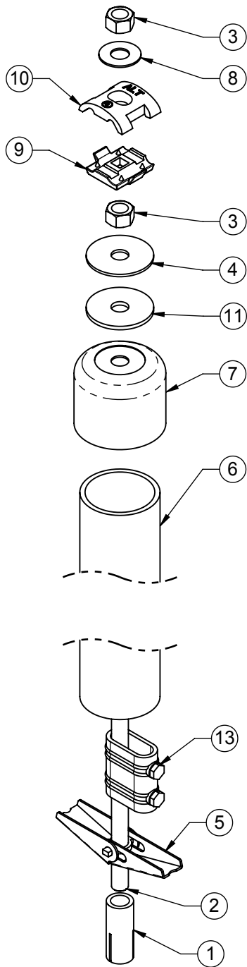
ISO VIEW
