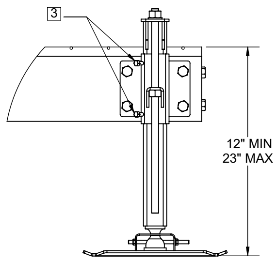
DETAIL B
